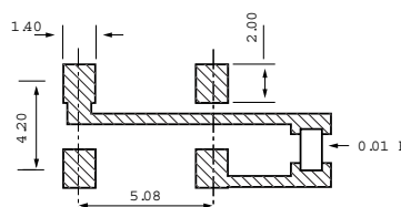
Figure 2) Land Pattern
